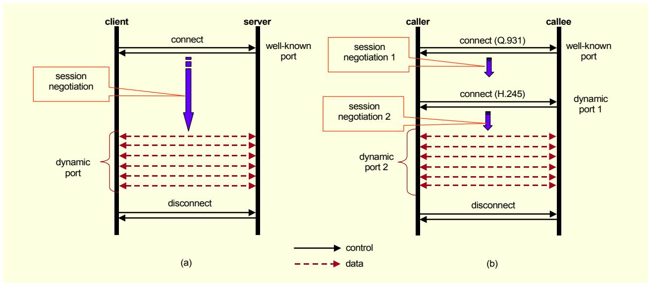
Fig. 1. A multimedia service control and data session: (a) RealMedia, QuickTime, WMT, SIP, (b) H.323.
