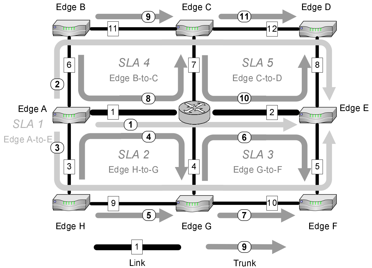
Fig. 4 Network topology, SLAs and trunk deployment for simulation
