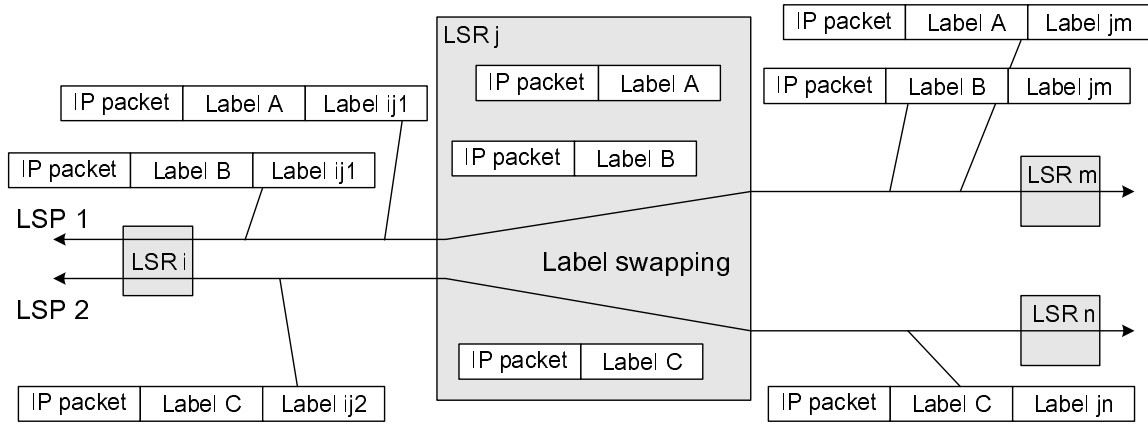
Fig. 3 Two layer label stacking to support virtual networks
