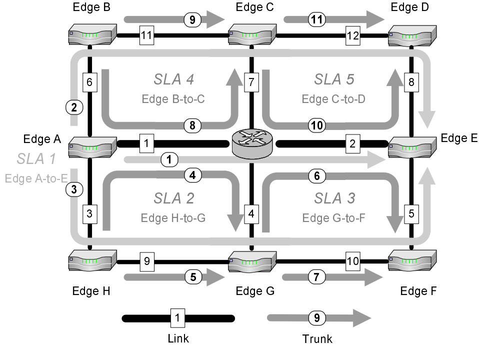
Fig. 4 Network topology, SLAs and trunk deployment for simulation
