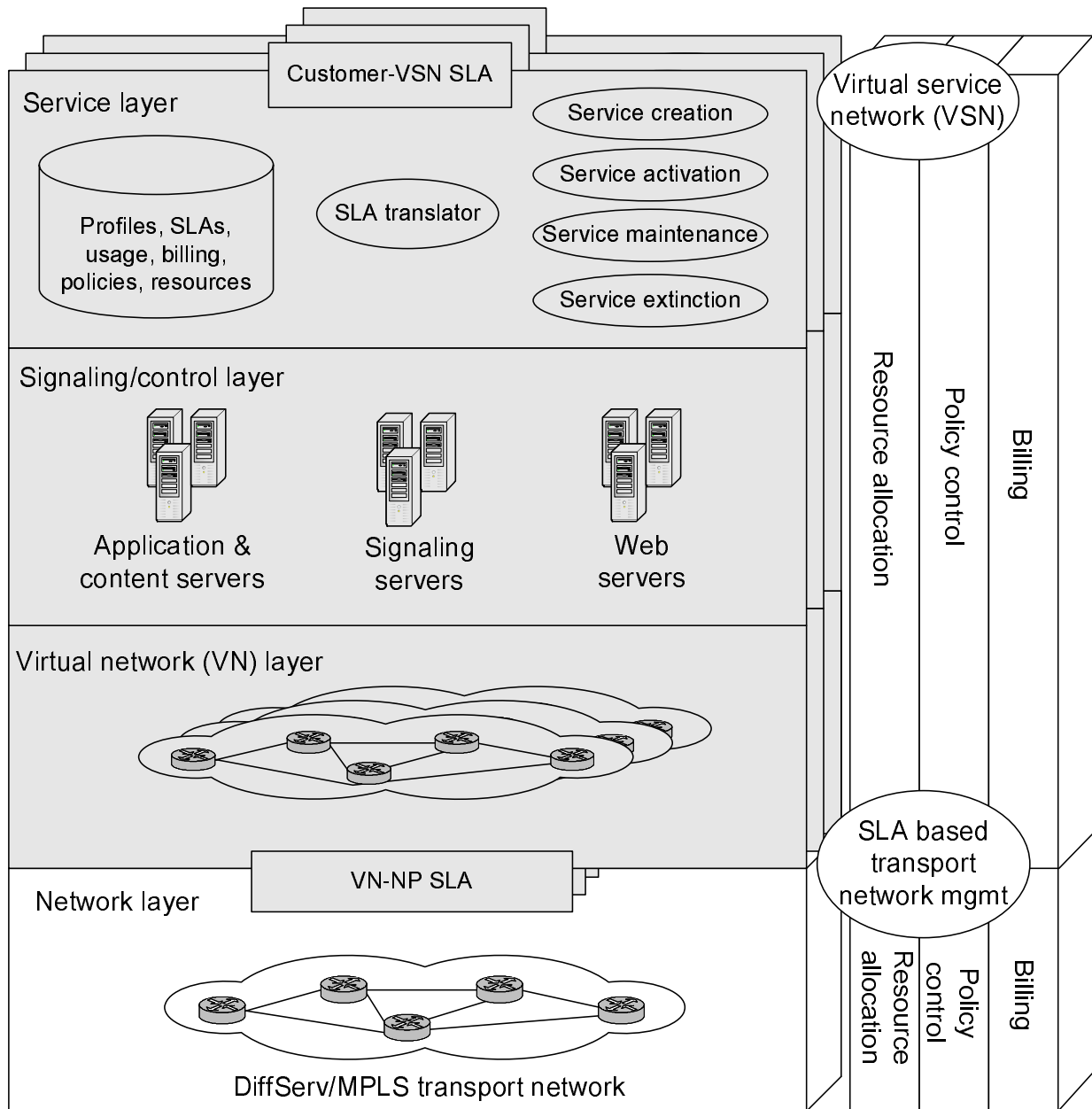
Fig. 1 Virtual network based service and network management architecture
