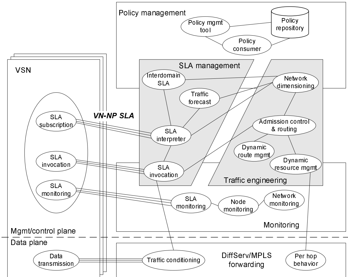
Fig. 2 VTEQUILA architecture for a DiffServ/MPLS network supporting virtual networks
