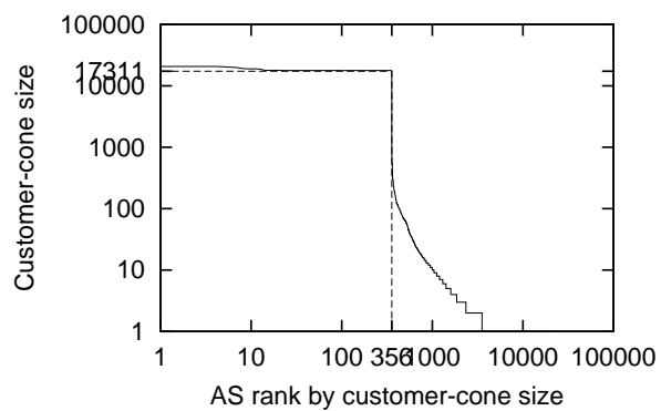
Figure 11. Customer-cone size of ASes.
