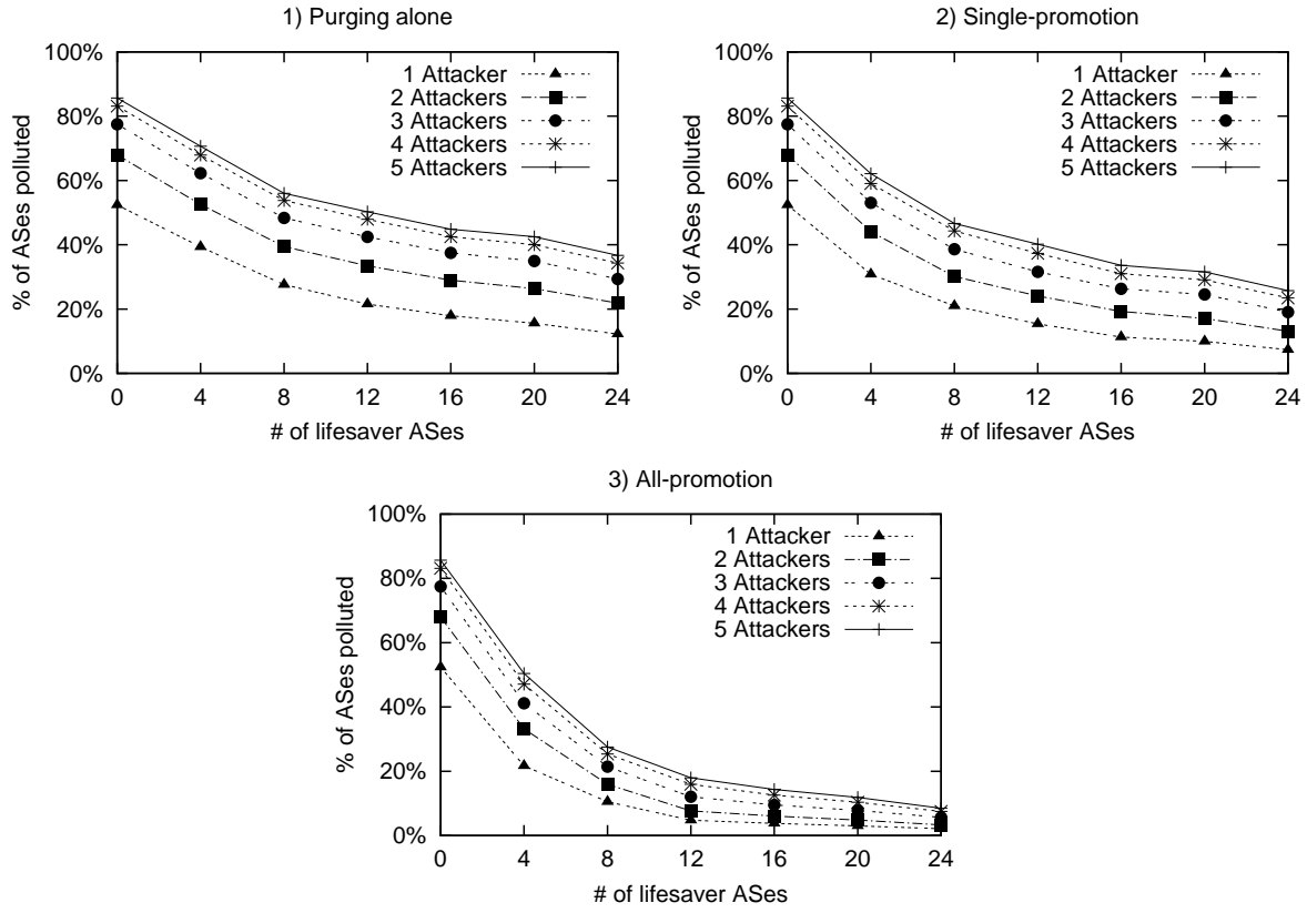
Figure 5. Pollution of a random colluding hijack when (1) all lifesavers perform purging, (2) single lifesaver performs promotion in addition to purging, (3) all lifesavers perform promotion in addition to purging.
