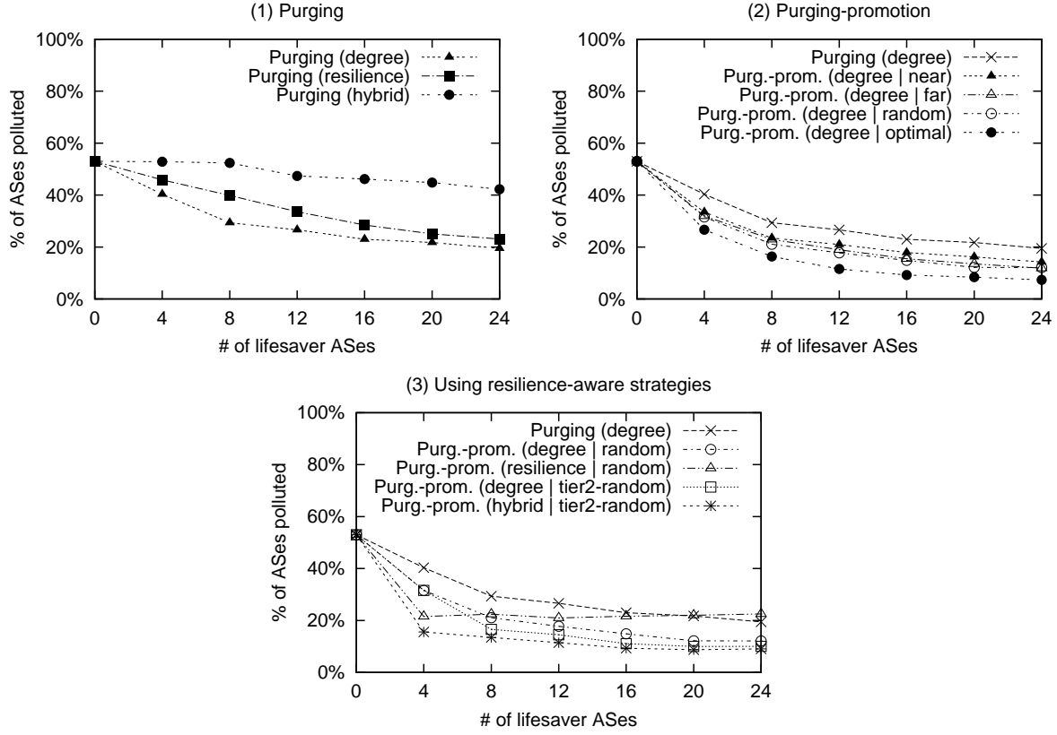
Figure 3. Pollution of a random prefix hijack when a number of lifesavers perform (1) bogus route purging, (2) purging-promotion using degree-based strategies, (3) purging-promotion using resilience-aware strategies.
