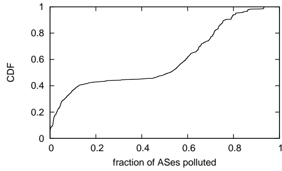
Figure 8. The polluted ASes under detection evasion.
